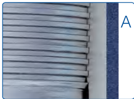
Flank-to-flank contact thread Taper=1 : 16 4-1/2in ~8-5/8in: 5TPI 9-5/8in~13-3/8in: 4TPI
