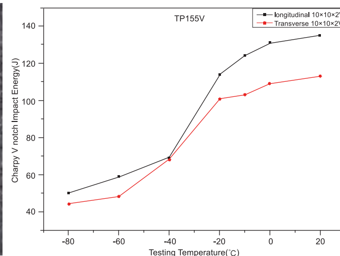
Typical Longitudinal and Transverse Impact Properties
